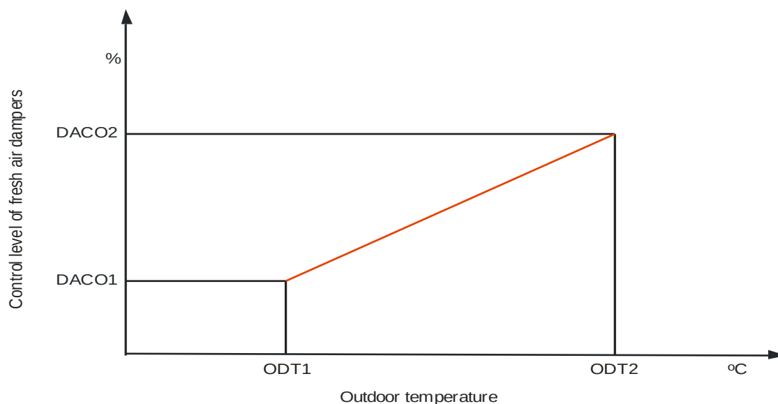
Mixing chamber dampers control description in AUTO mode
